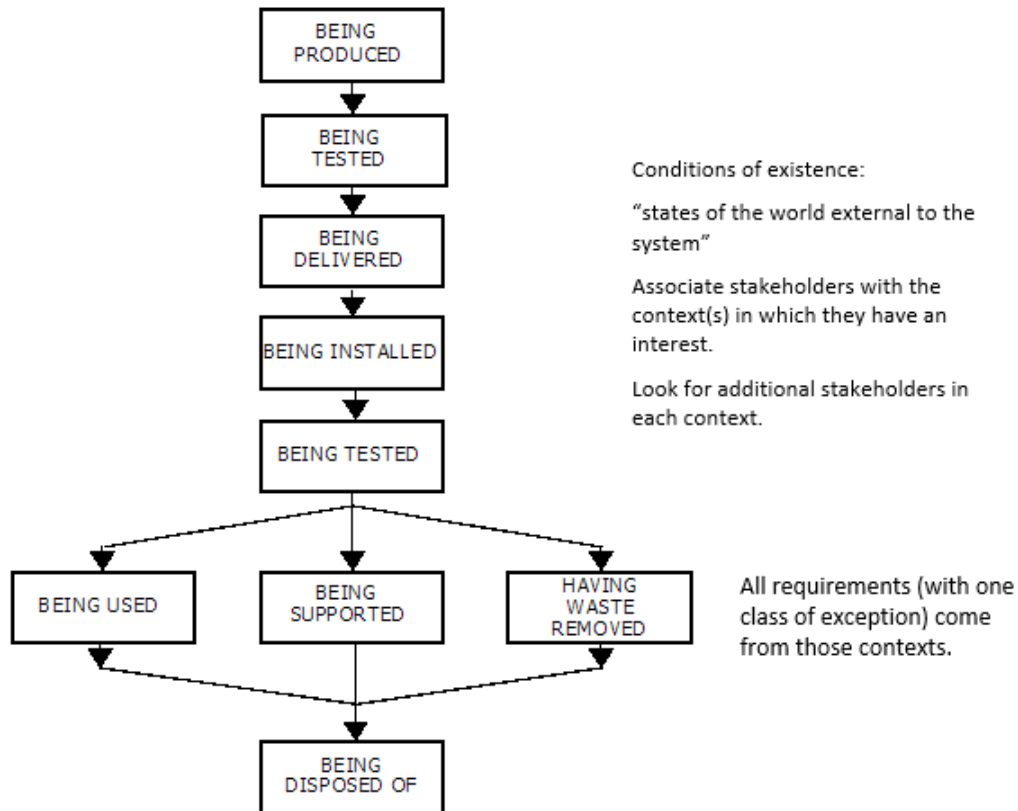
Figure 2: Context Flow Diagram
