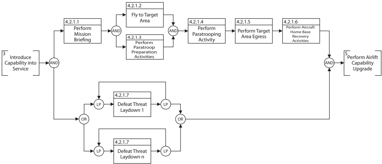
Figure 5: Functional Flow Block Diagram
