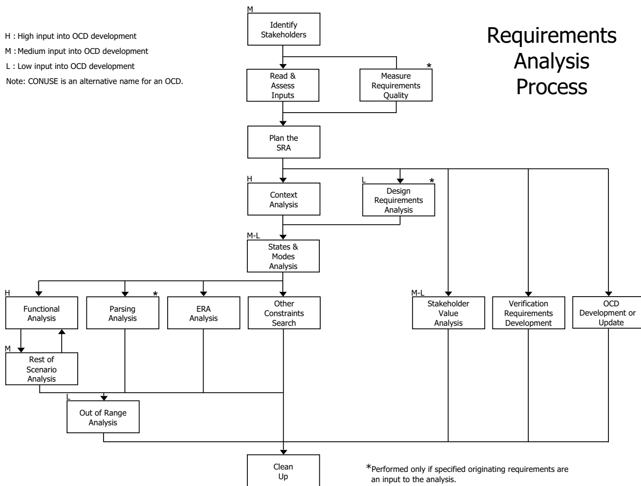
Figure 1: An Effective Requirements Analysis Process
