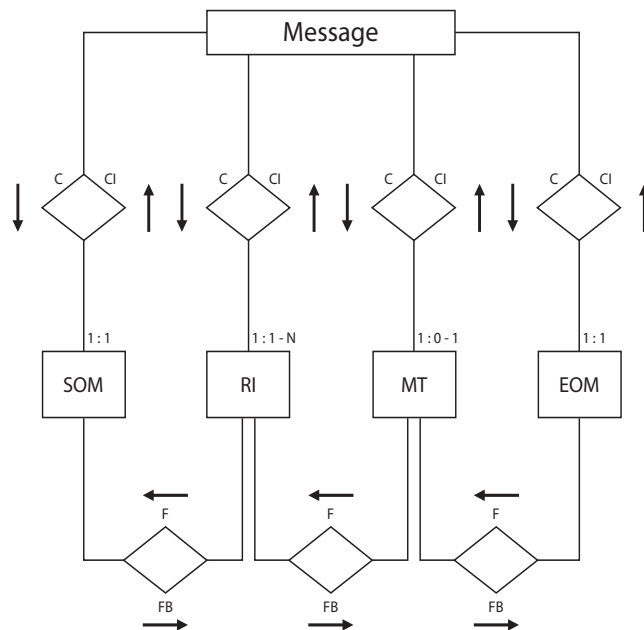
Figure 6: Entity Relationship Attribute Diagram
