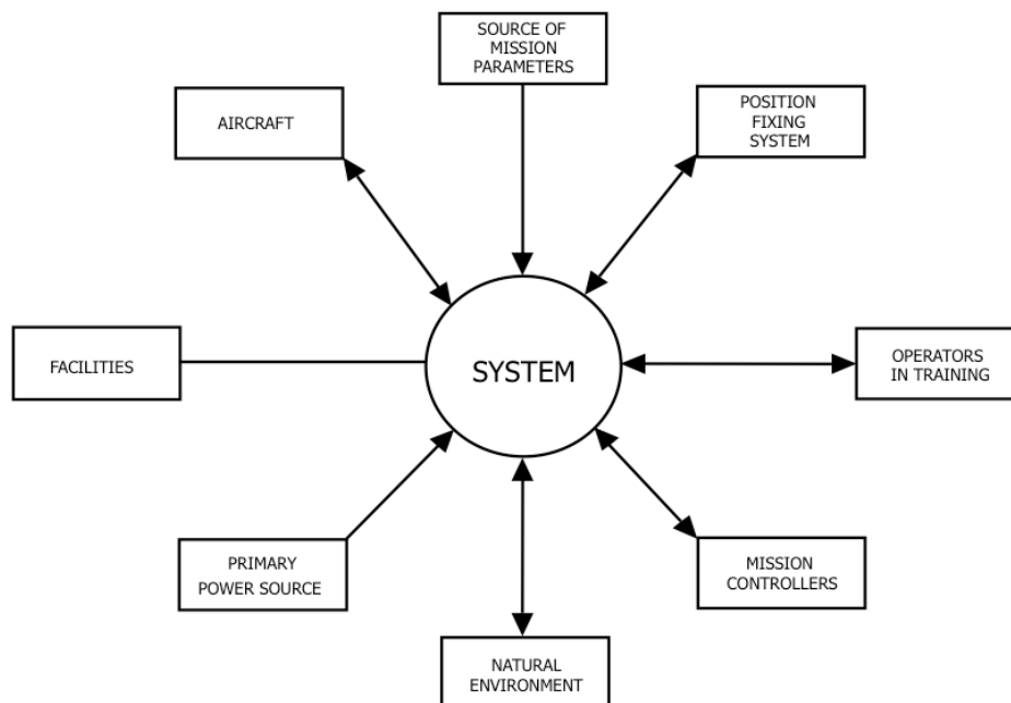
Figure 3: Context Diagram
