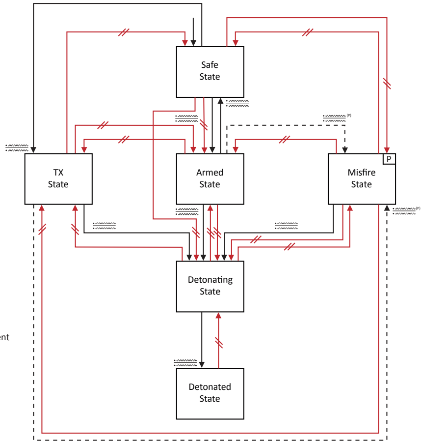
Figure 4: States Transition Diagram
