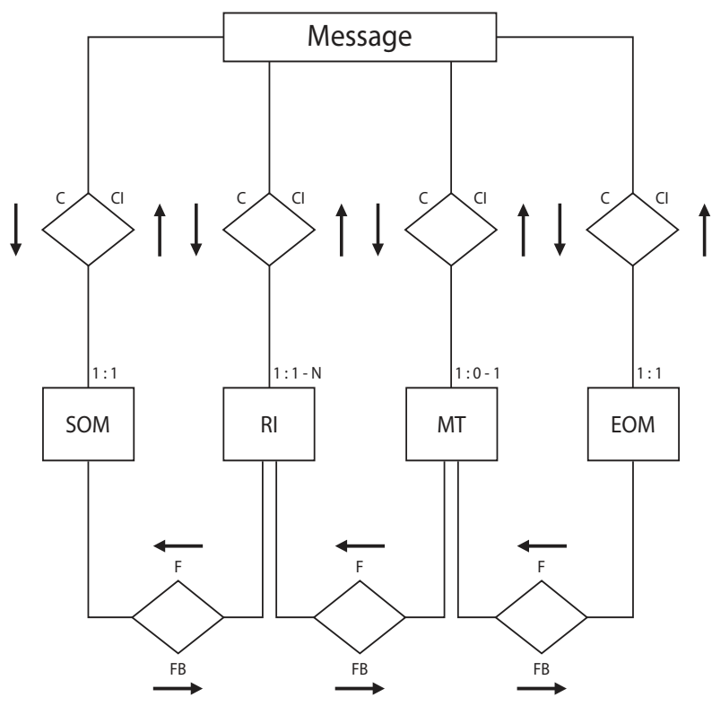
Figure 6: Entity Relationship Attribute Diagram
