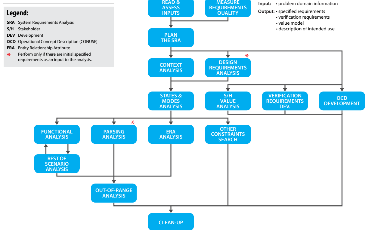
Figure 1: An Effective Requirements Analysis Process
