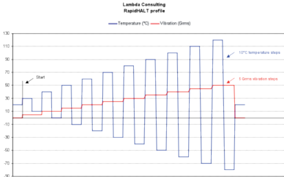
Figure 2: Test profile used in HALT
